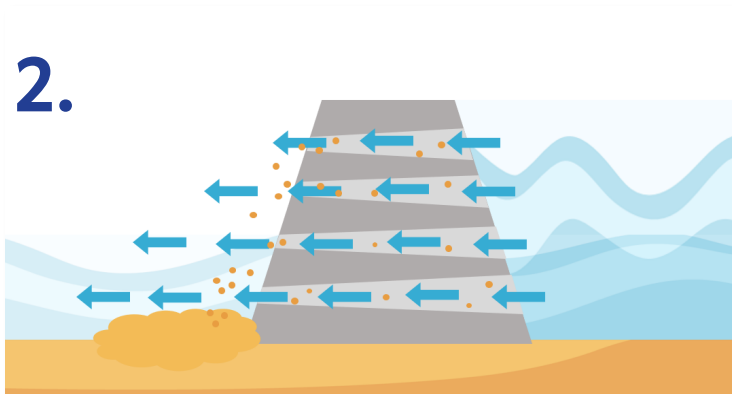
Wave action carrying and depositing sand
